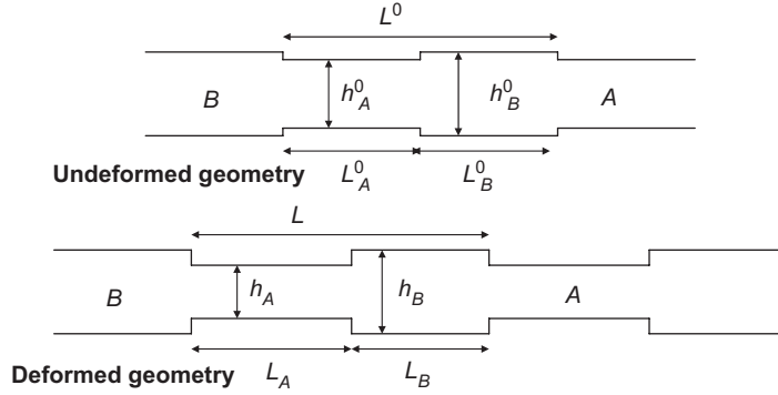
Fig. 10. Undeformed and deformed geometry of the two-state model for dynamic neck growth under overall stretching.
