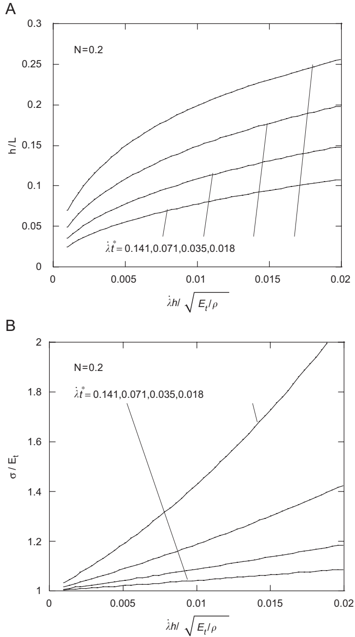
Fig. 9. Undulation wavelength (A) associated with the minimum stress (B) required to achieve four undulation growth times, \lambda t^* , under uniform dynamic stretching specified by \lambda h l \sqrt{E_t / \rho} , as determined by the analysis of Shenoy and Freund (1999). In the current state, E_t is the tangent modulus, h is the plate thickness, and L is the wavelength of the sinusoidal undulation.
